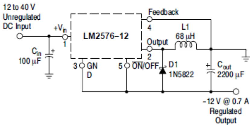
Figure 26. Inverting Buck-Boost Develops -12 V
