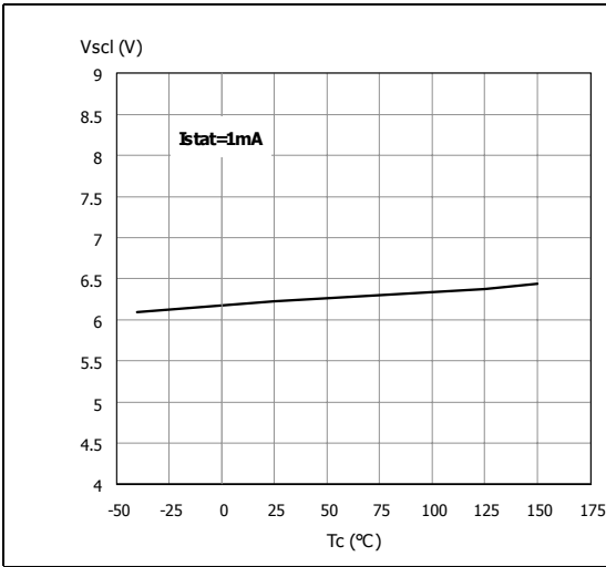
Figure 16. Status clamp voltage
