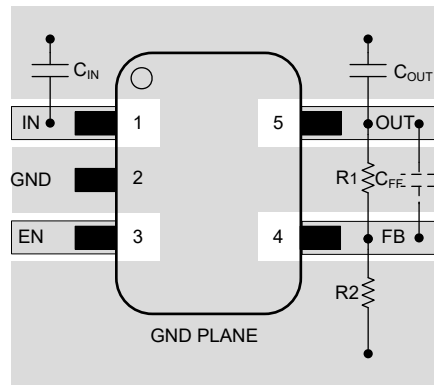
Figure 8-8. Layout Diagram
