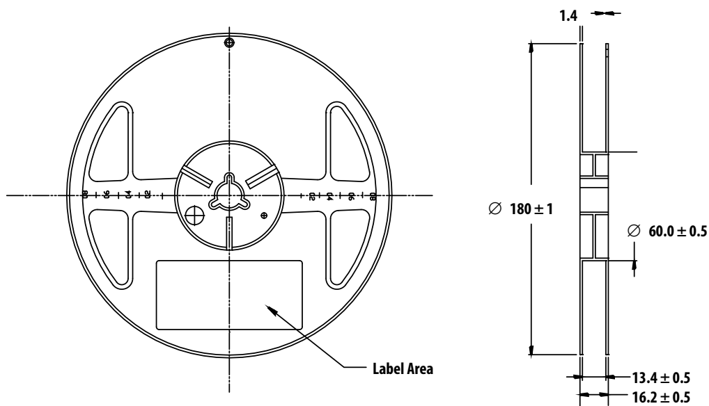
Figure 14. Reel Dimension
