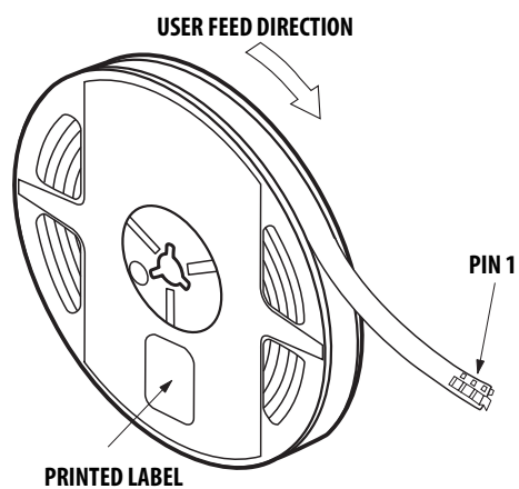
Figure 15. Reeling Orientation
