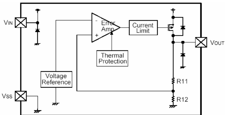
XC6216D/XE6216D Series (SOT-89, SOT-223, TO-252)
