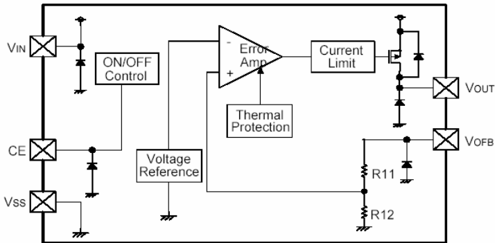
XC6216C/XE6216C Series (SOT-25, SOT-89-5, USP-6C)
