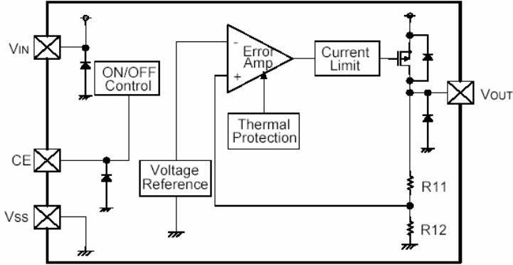
XC6216B/XE6216B Series (SOT-25, SOT-89-5, USP-6C)
