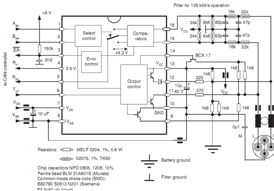
Figure 6-2. Application Circuit
