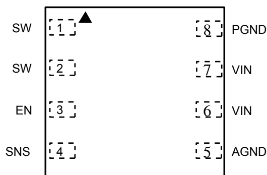
(Top View) 2mm x 2mm Thin MLF (MT)
