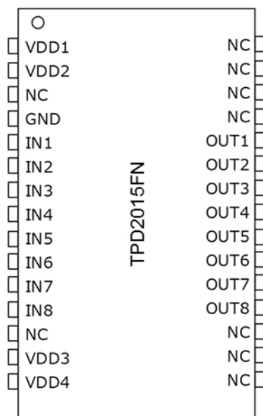
Fig. 4.1 Pin assignments
