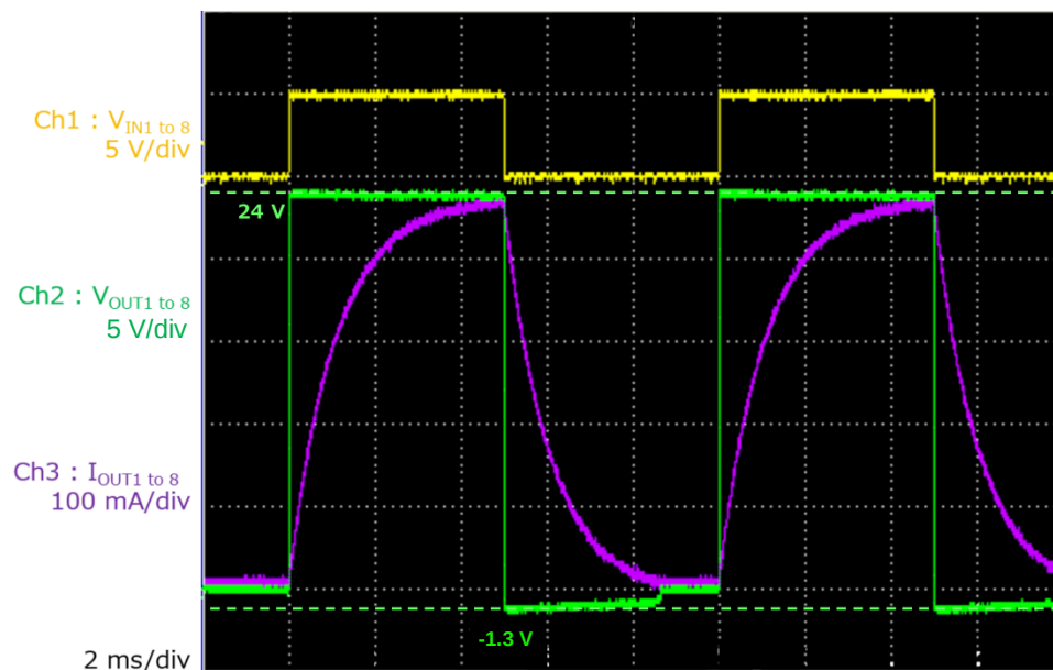
Fig. 3.1 Normal operation waveform
