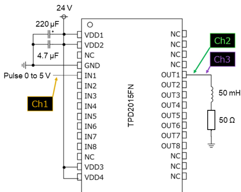
Fig. 3.2 Example of normal operation circuit
