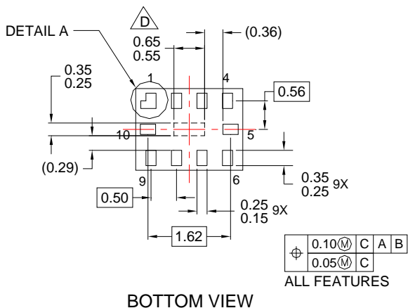
Figure 17. 10-Lead MicroPak, 1.6 x 2.1mm
