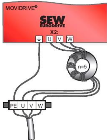
Abb. 4-7 Ferrit-Ringkern 29
