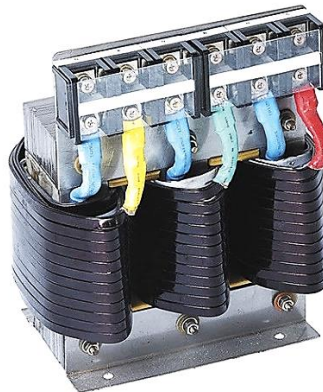
Abb. 4-5 Oberwellenfilter
