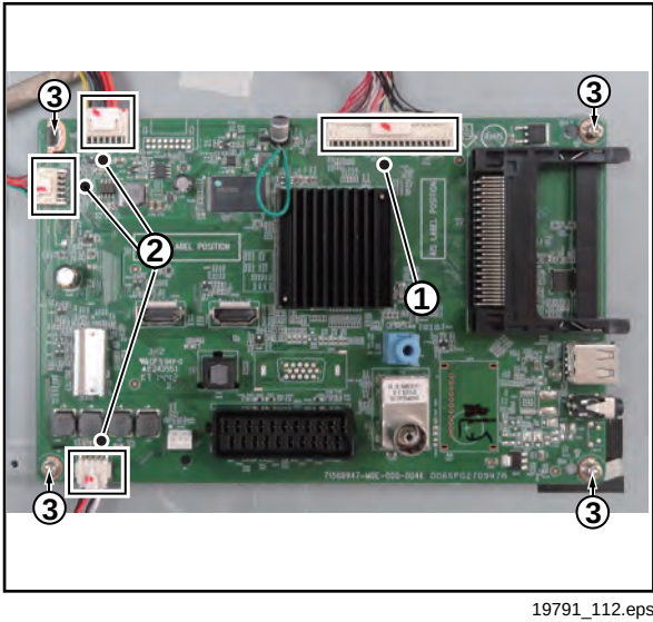
Figure 4-20 SSB removal
