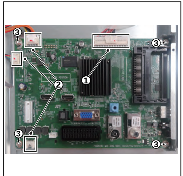
Figure 4-34 SSB removal
