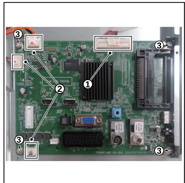
Figure 4-17 SSB removal
