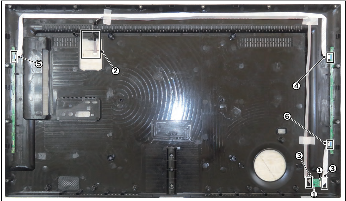
Figure 4-29 Rear cover removal[2]
