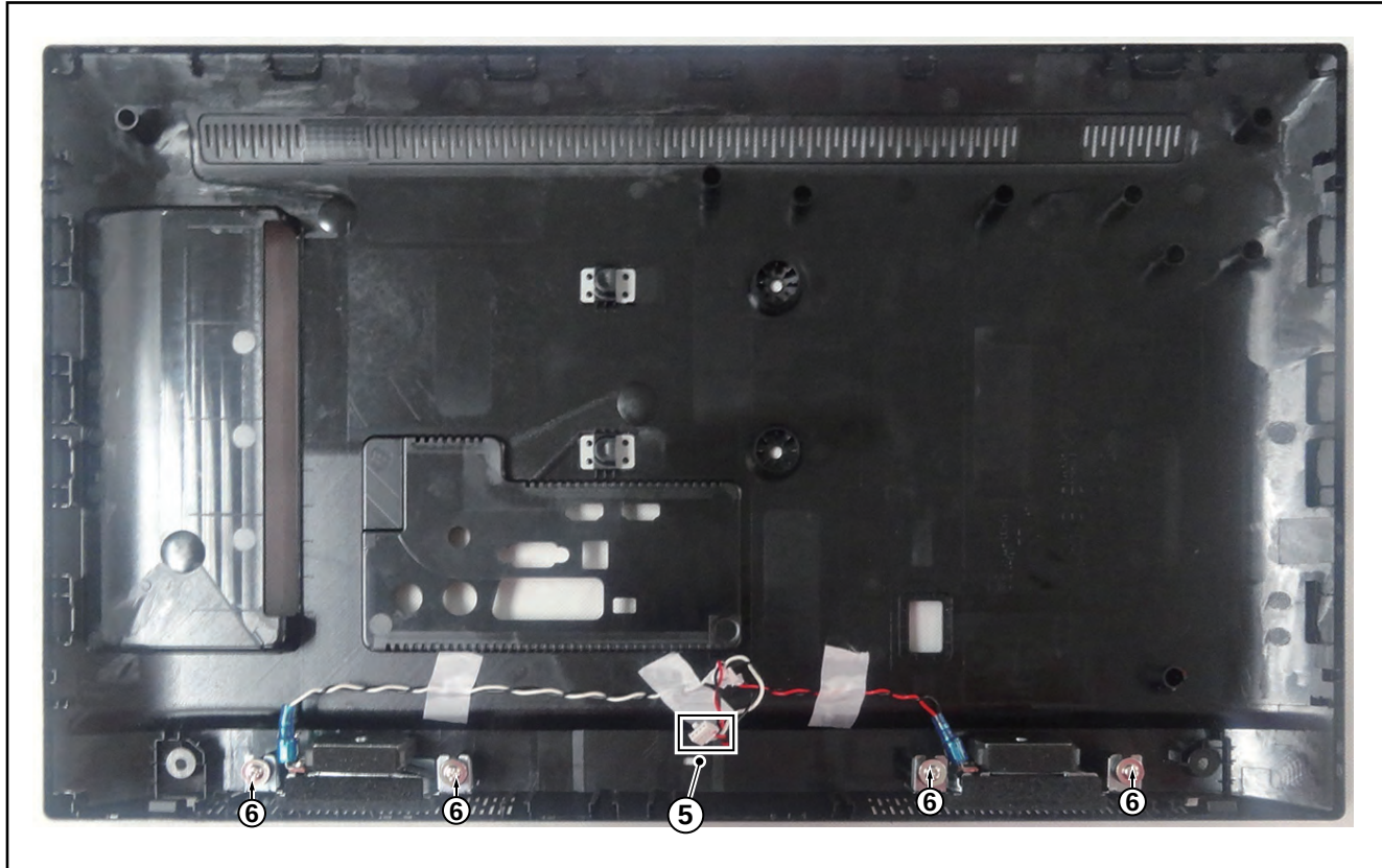
Figure 4-16 Speakers removal
