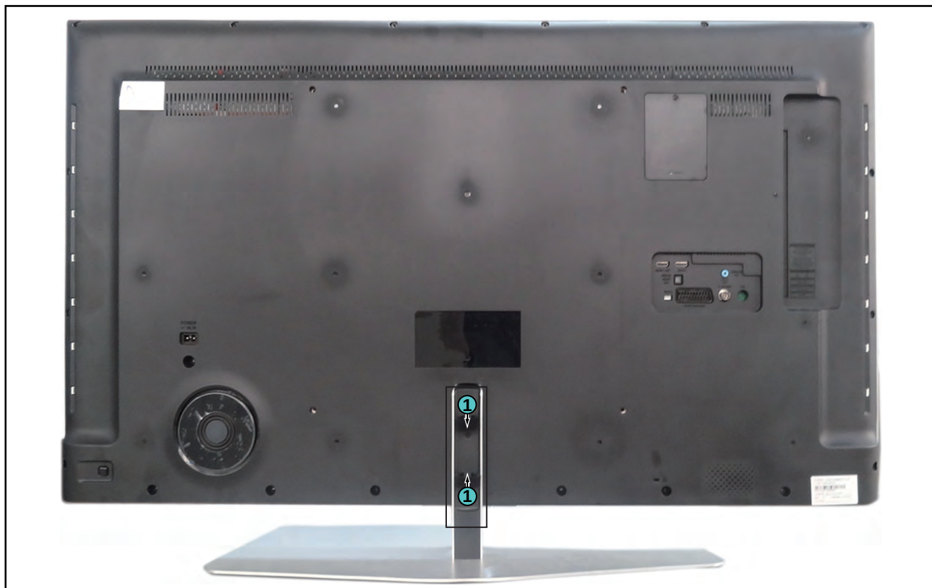
Figure 4-26 Stand removal[1]
