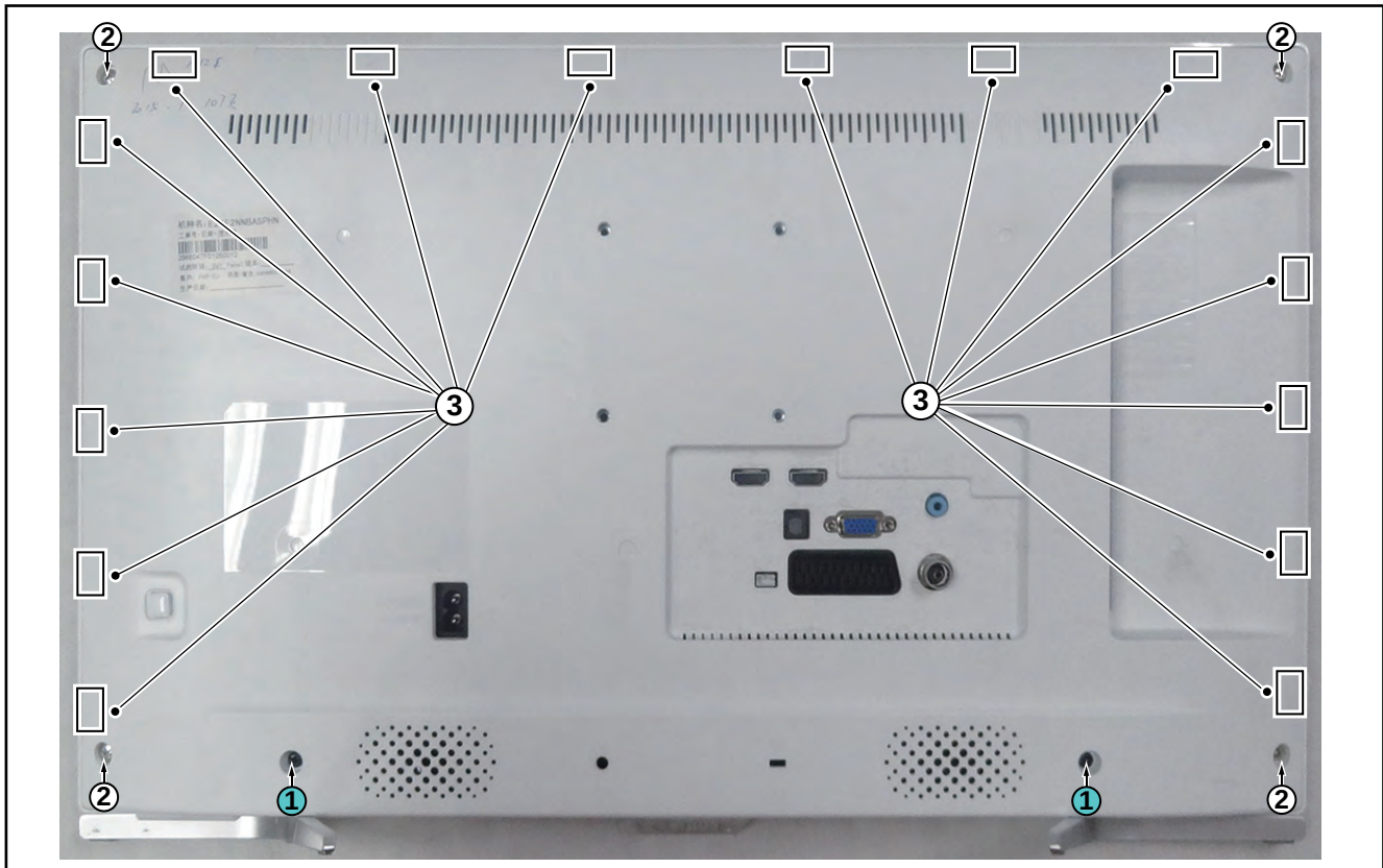
Figure 4-32 Rear cover removal
