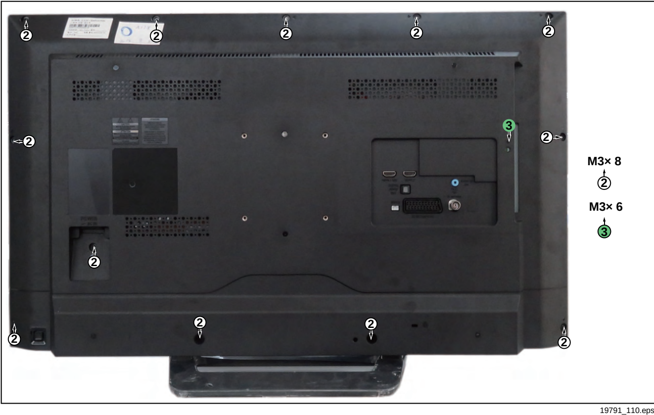
Figure 4-19 Rear cover removal
