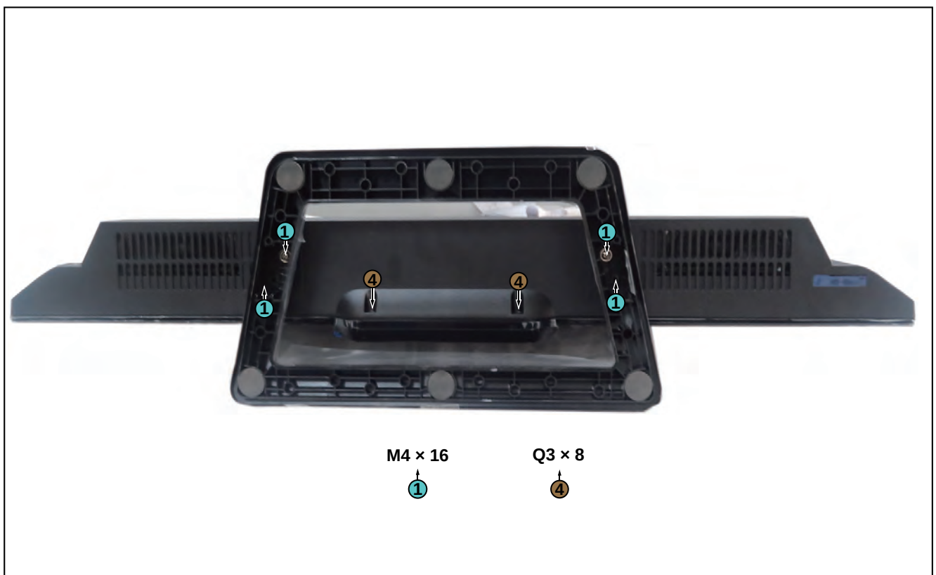
Figure 4-18 Stand removal
