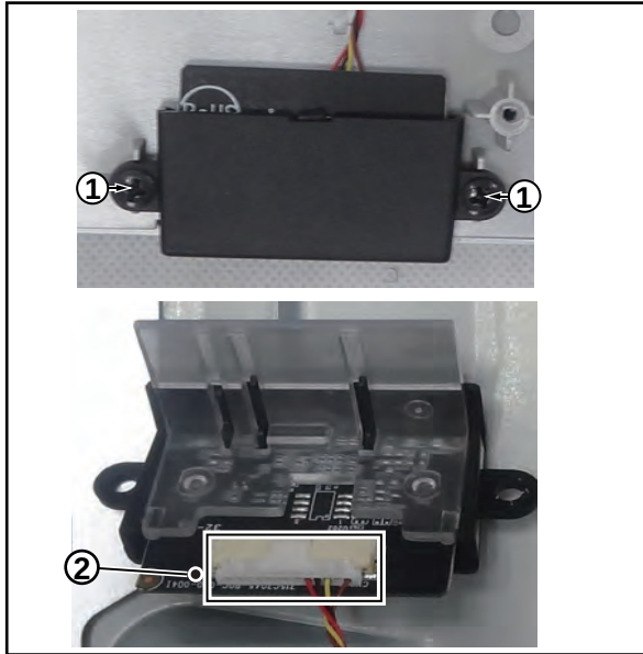
Figure 4-31 IR/LED Board removal
