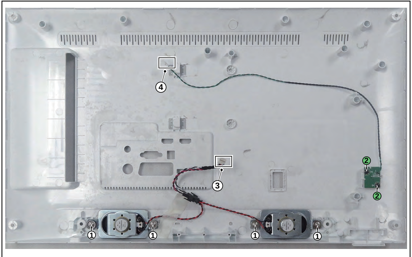
Figure 4-33 Speakers and Keyboard removal
