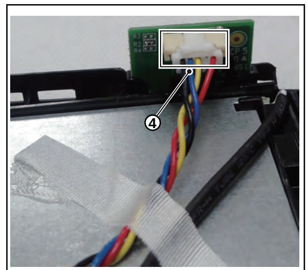
Figure 4-15 IR/LED Panel removal
