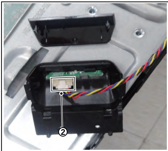
Figure 4-25 IR/LED Board removal[2]
