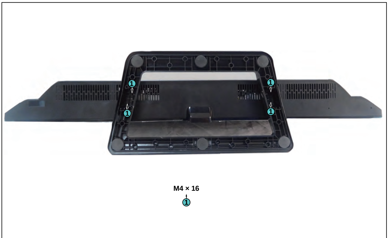
Figure 4-21 Stand removal
