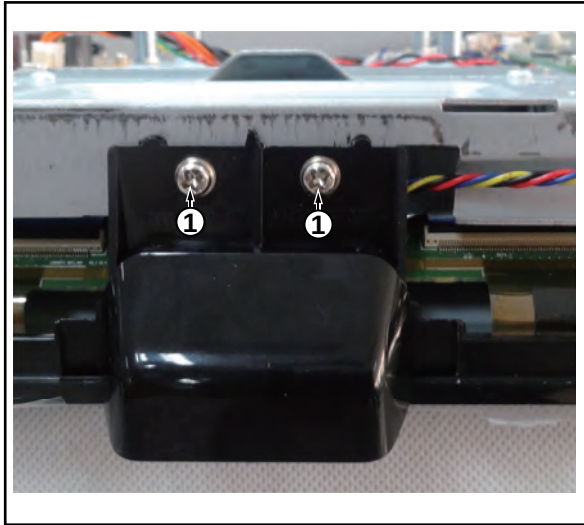
Figure 4-24 IR/LED Board removal[1]
