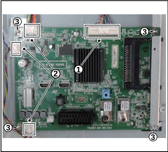
Figure 4-23 SSB removal
