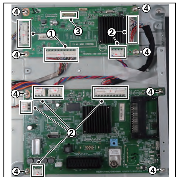
Figure 4-30 SSB + FRC Board removal
