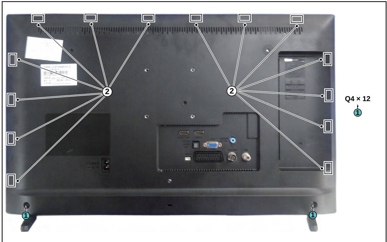
Figure 4-13 Rear cover removal [1]
