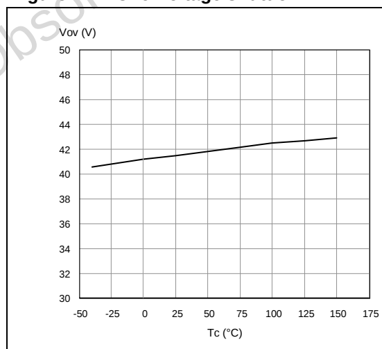
Figure 11. Overvoltage shutdown
