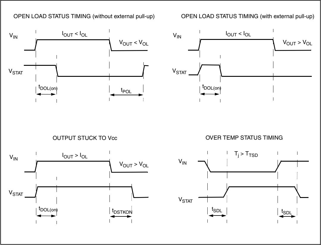
Figure 4. Status timings
