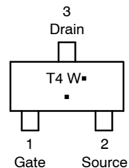
SC-70/SOT-323 CASE 419 STYLE 8
