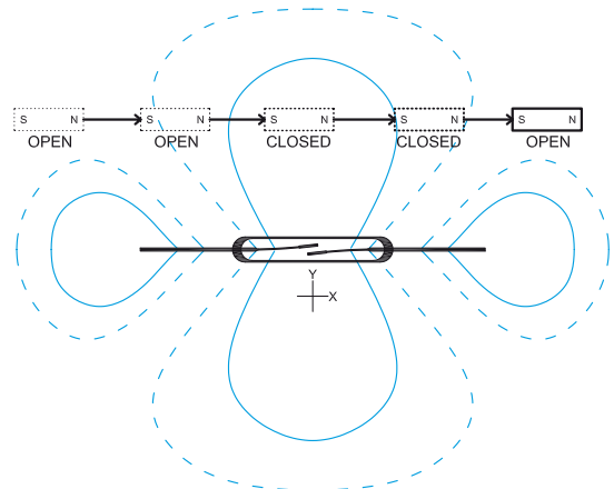
Position and movement resulting in one closure and one opening.
