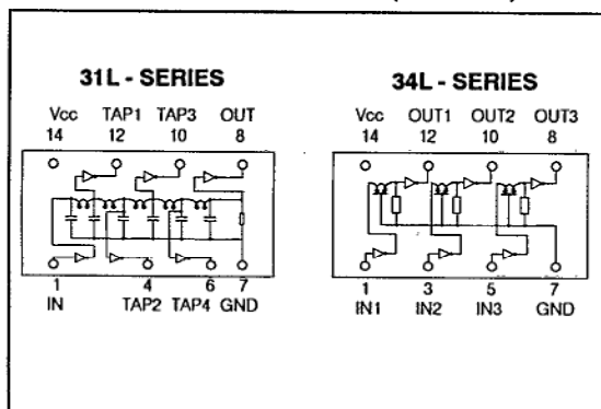
DUAL-IN-LINE PACKAGE (TOP VIEW)
