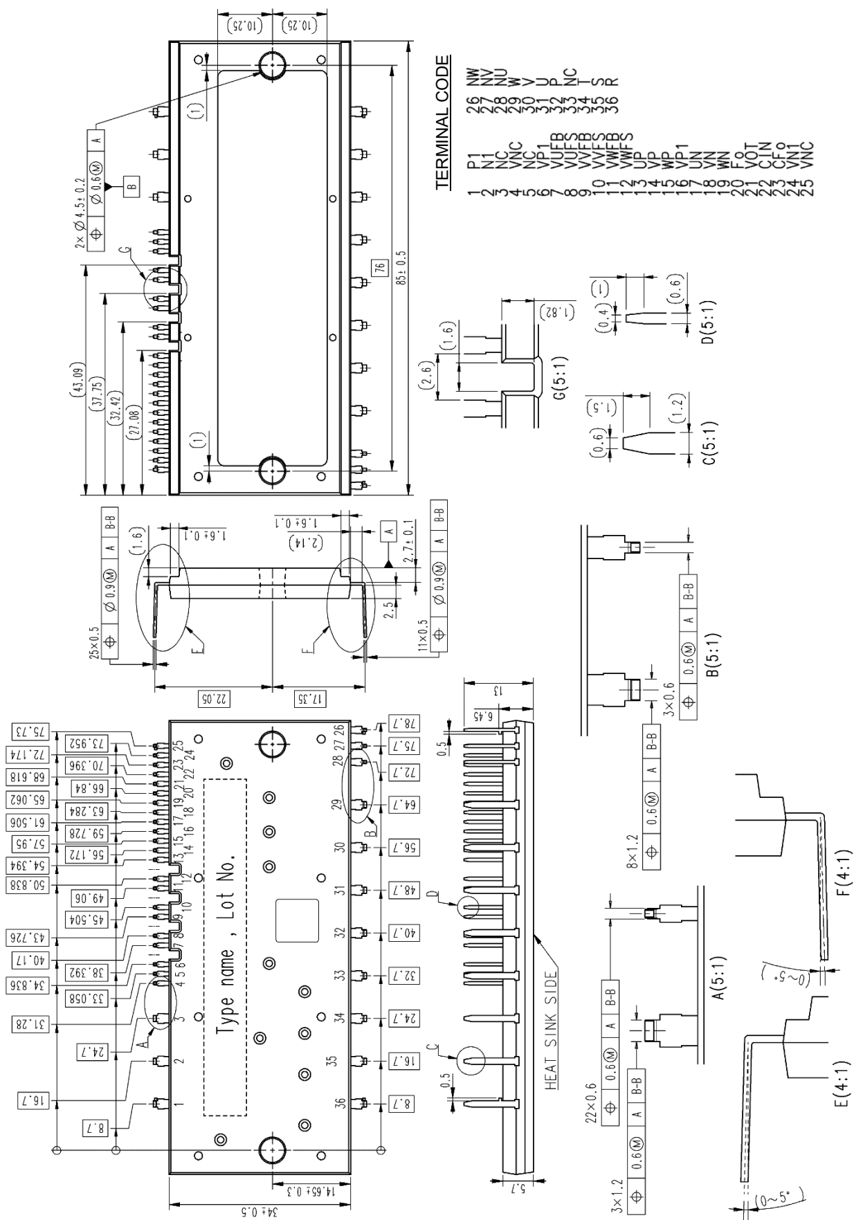
Dimensions in mm
