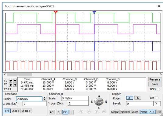
Fig. 6. 5 frequency divider circuit simulation results.
