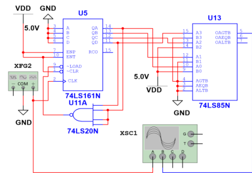
Fig. 3. 10 Frequency division circuit design.
