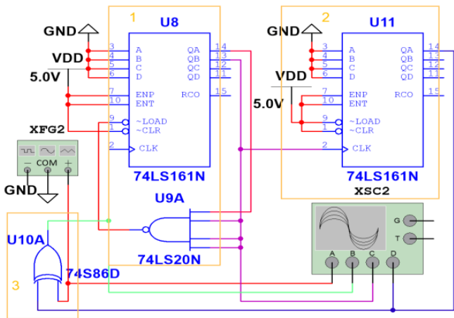
Fig. 7. 3.5 Frequency division circuit design.
