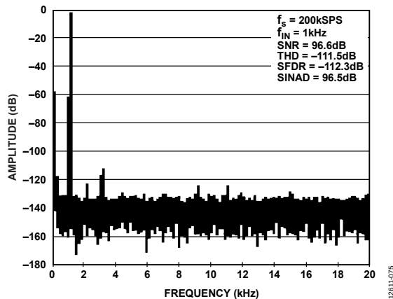
Figure 75. FFT for Driving a Differential Converter, -0.5 \text{ dBFS}
