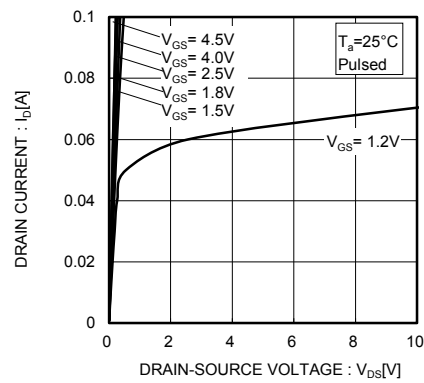
Fig.2 Typical Output Characteristics ( II )
