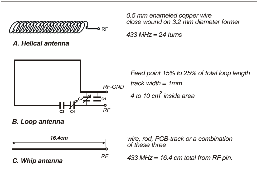
Fig.8: Antenna
