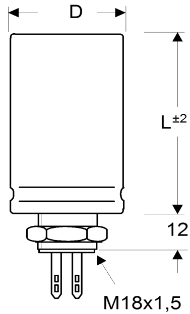
Fig2: SZ for stud mounting
