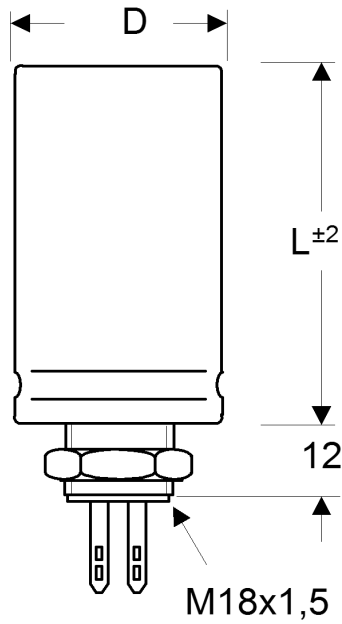
Fig1: S for clamp mounting
