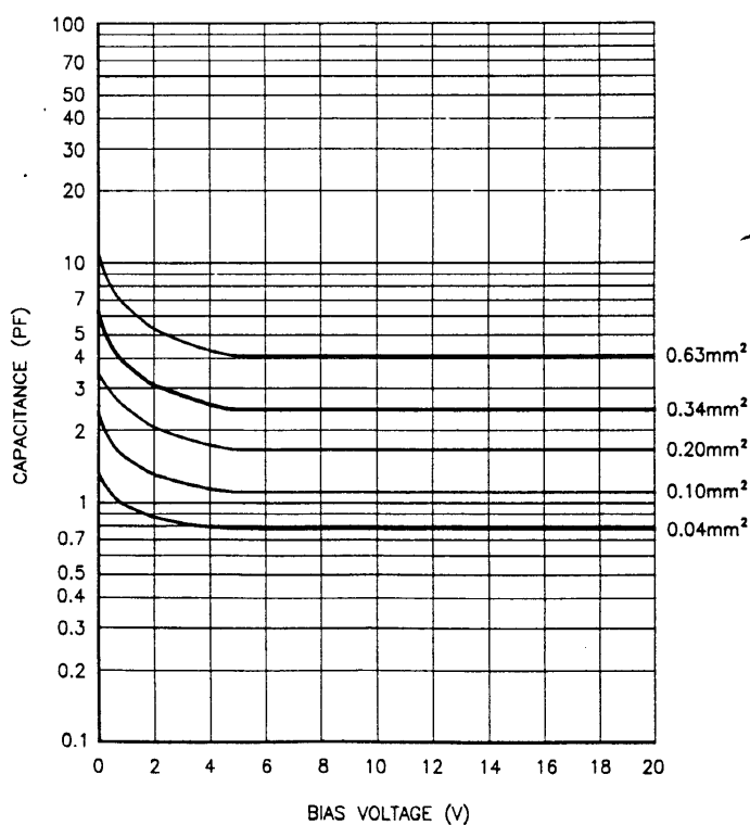
Series AEPX - Typical Capacitance versus Bias Voltage and Active Area
