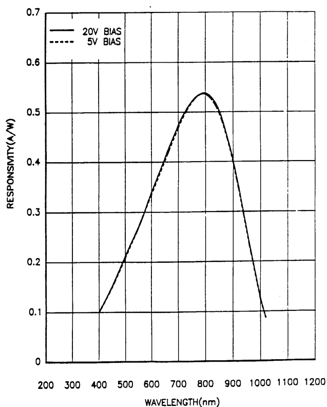
Series AEPX - Typical Spectral Response
