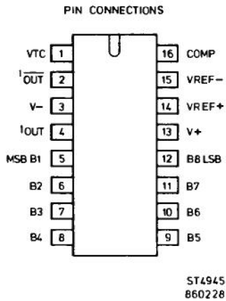
Figure 3.16 Pin connections
