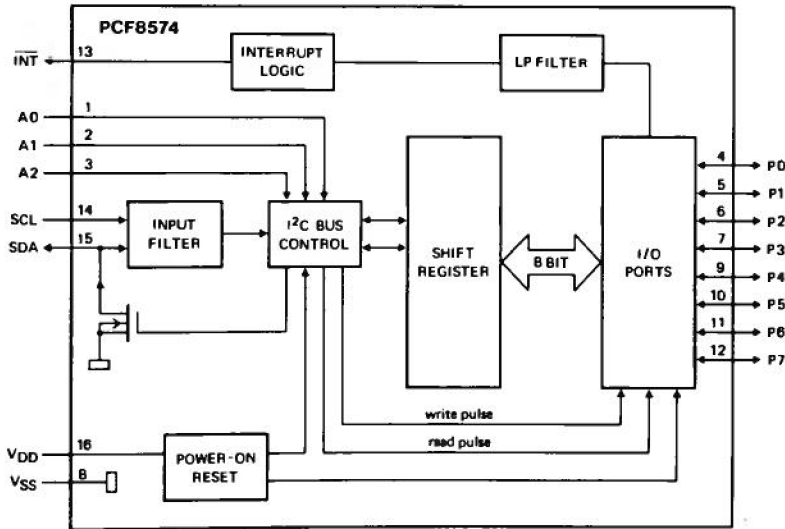
Figure 3.24 Block diagram
