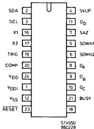
Figure 3.22 Pinning
