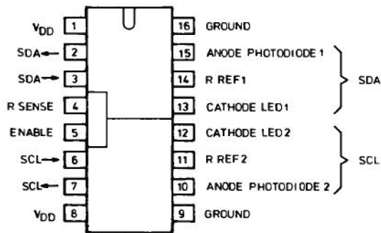
Figure 3.20 Pinning
