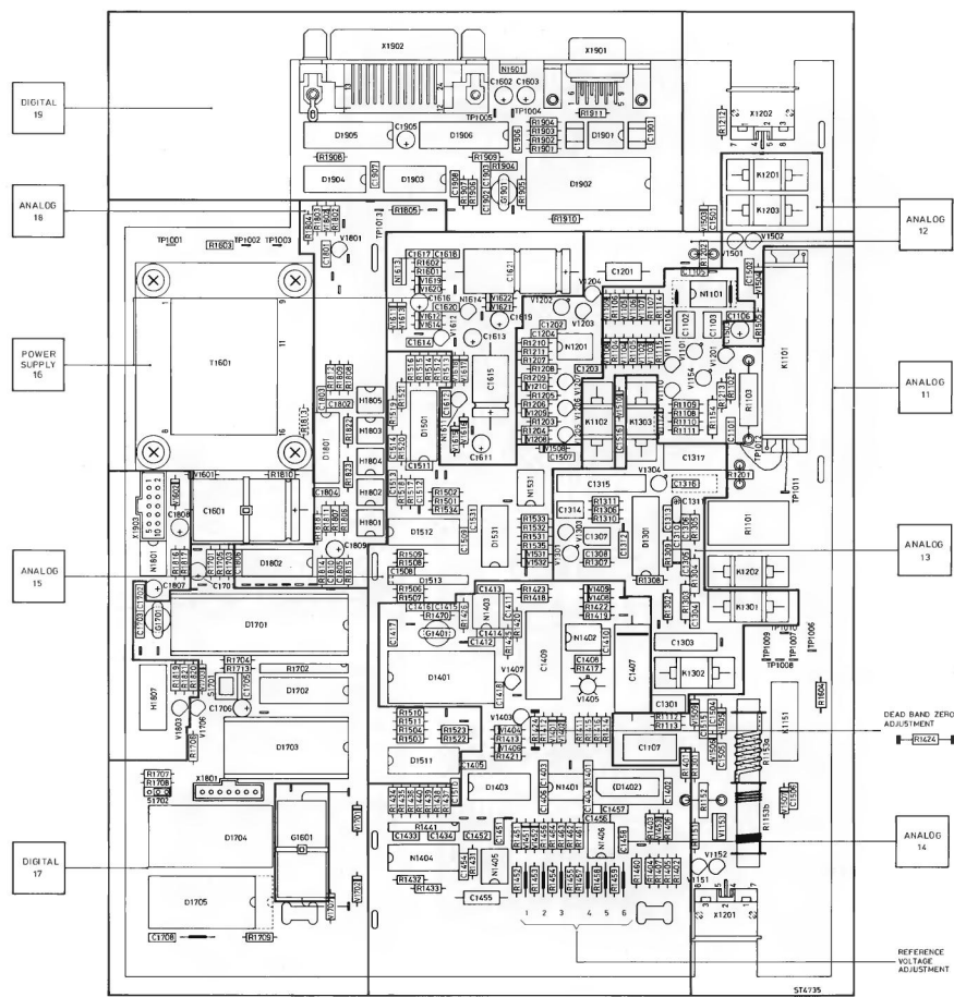
Figure 9-12 Main pcb parts location (version 4022 325 8051.3, almost equal to version 4022 325 8051.2) ST484 900126
