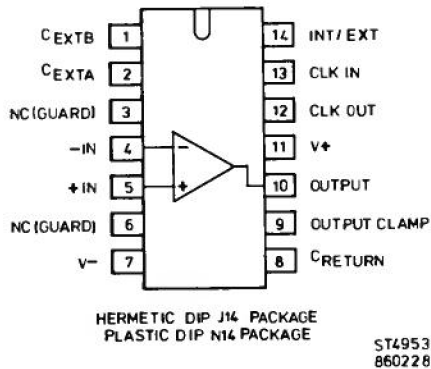
Figure 3.28 Pin connections
