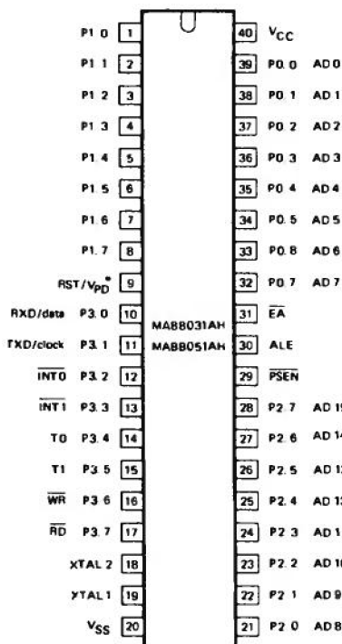
Figure 3.13 Pin Configuration
