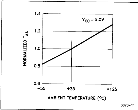
Normalized Access Time vs. Ambient Temperature
