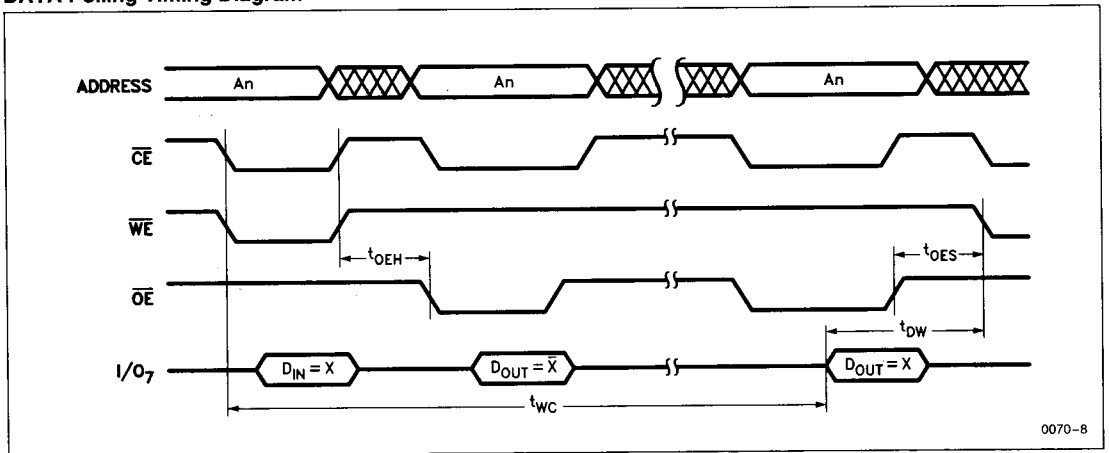
DATA Polling Timing Diagram(8)
