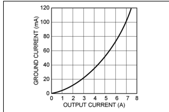
FIGURE 2-66: MIC2975x Ground Current vs. Output Current.
