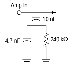
STATE 0: Normal operations with non-inverted charge polarity.
