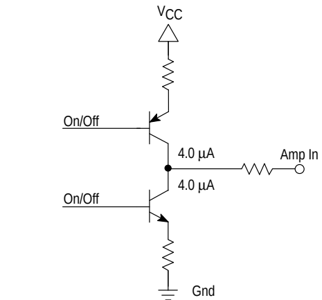
Figure 13. Output Configuration of the Phase Comparator
