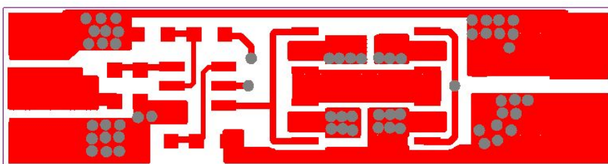
TOPLAYER
