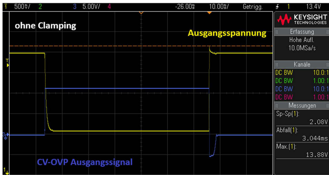
Abbildung 10: Without Anti-Windup and Clamping
