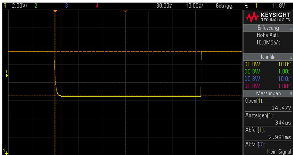
Abbildung 6: Switching CV to CC-Mode
