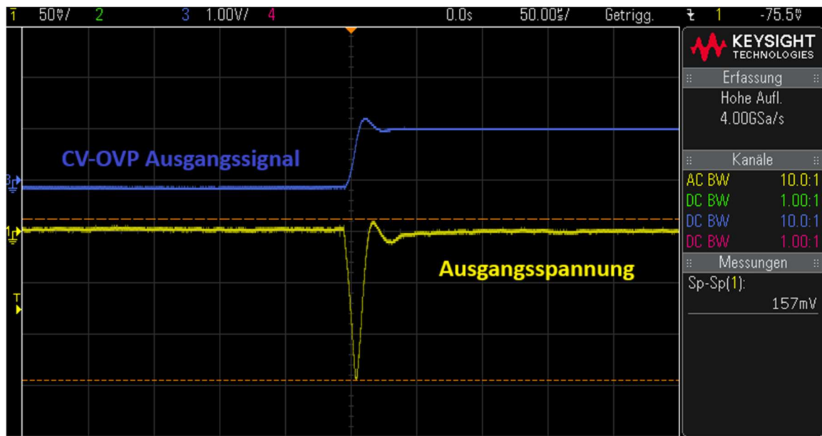
Abbildung 8: Transient Response: Turn on - 10 Ohm Resistor
