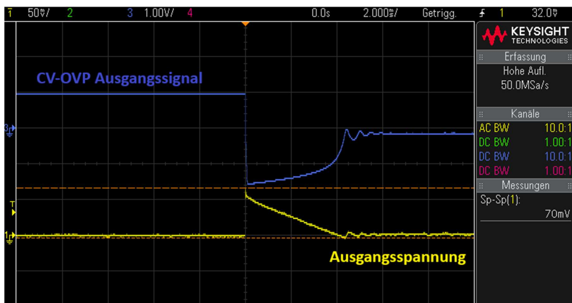
Abbildung 9: Transient Response: Turn off - 10 Ohm Resistor
