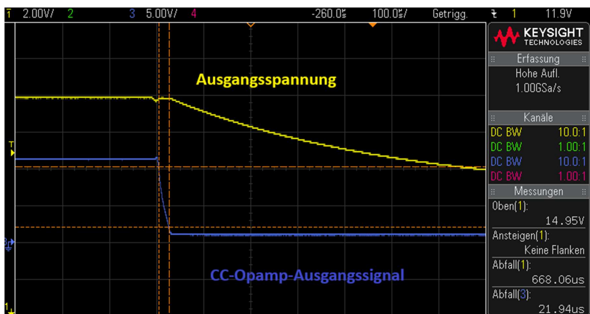
Abbildung 7: From CV to CC-Mode
