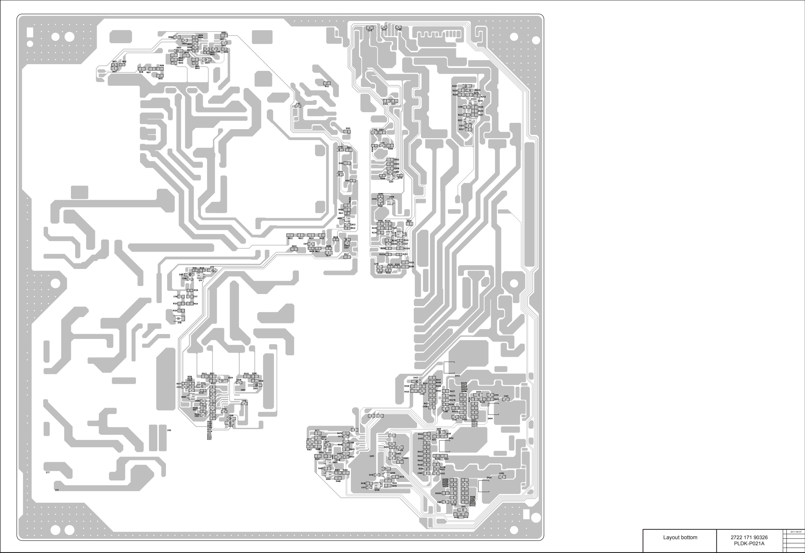
10-6-3 Layout bottom
