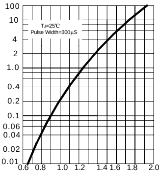
FIG.3 –TYPICAL FORWARD CHARACTERISTICS
