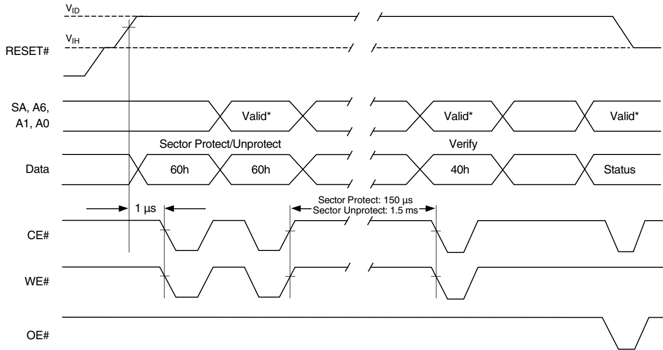
Figure 34. Sector/Sector Block Protect and Unprotect Timing Diagram
