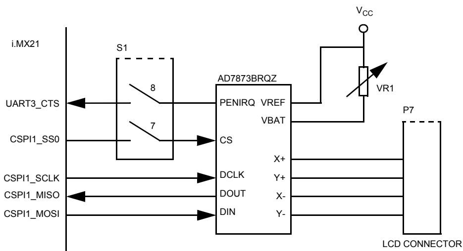
Figure 2-9. ADC Interface
