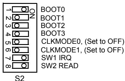
Figure 2-2. Switch S2
