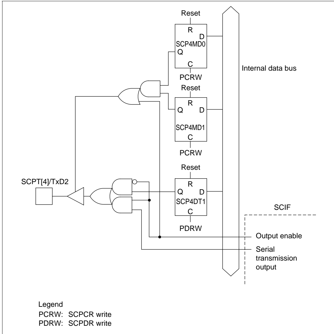
Figure 16.3 SCPT[4]/TxD2 Pin
