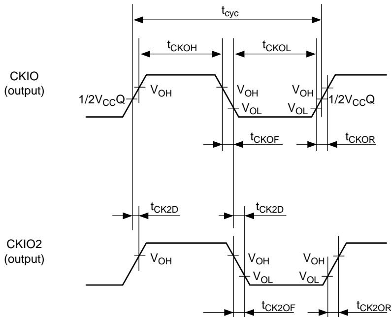
Figure 23.3 CKIO Clock Output Timing
