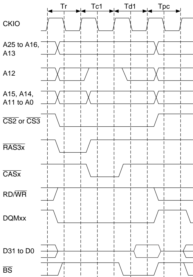
Figure 10.18 Basic Timing for Synchronous DRAM Single Read
