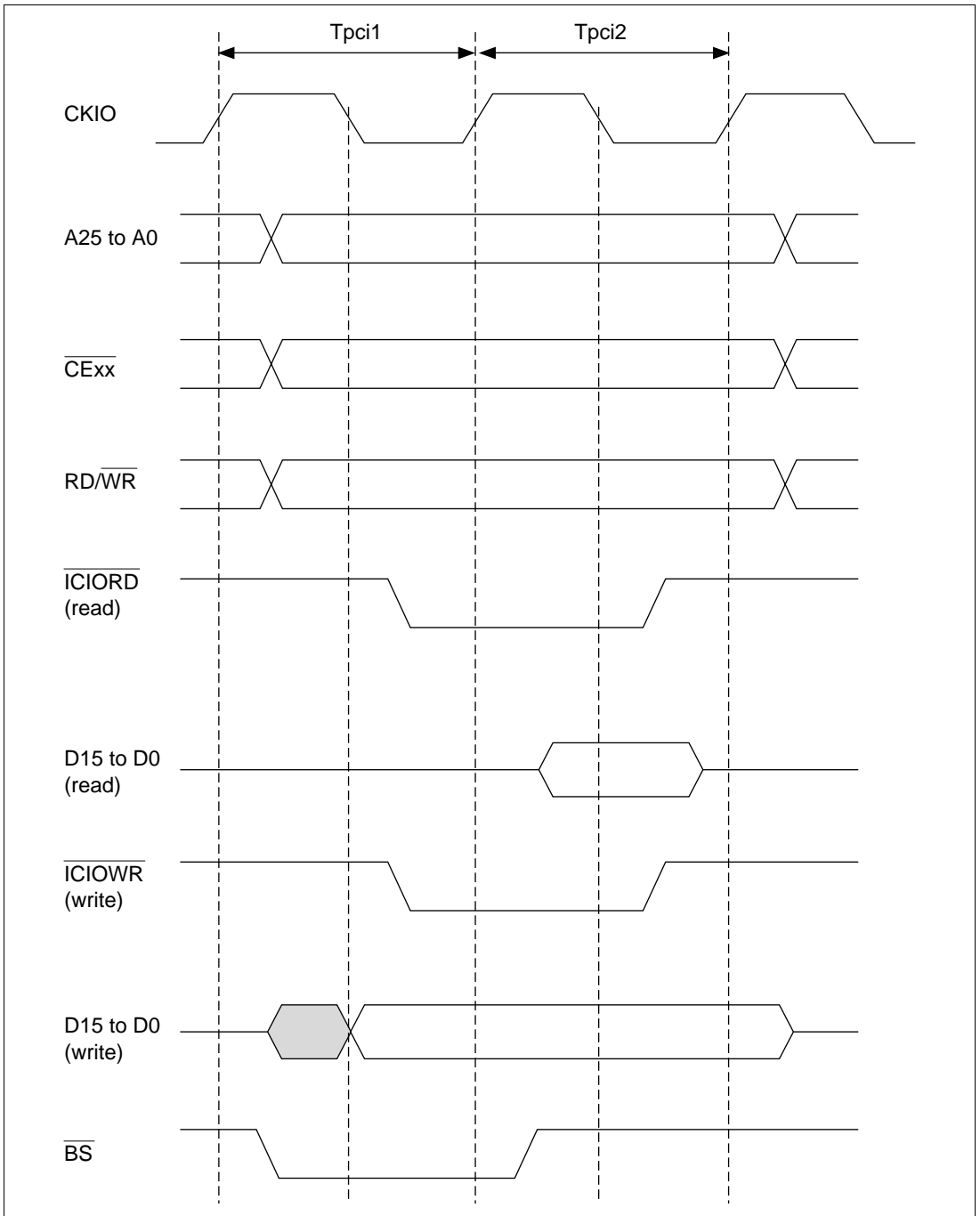
Figure 10.39 Basic Timing for PCMCIA I/O Card Interface
