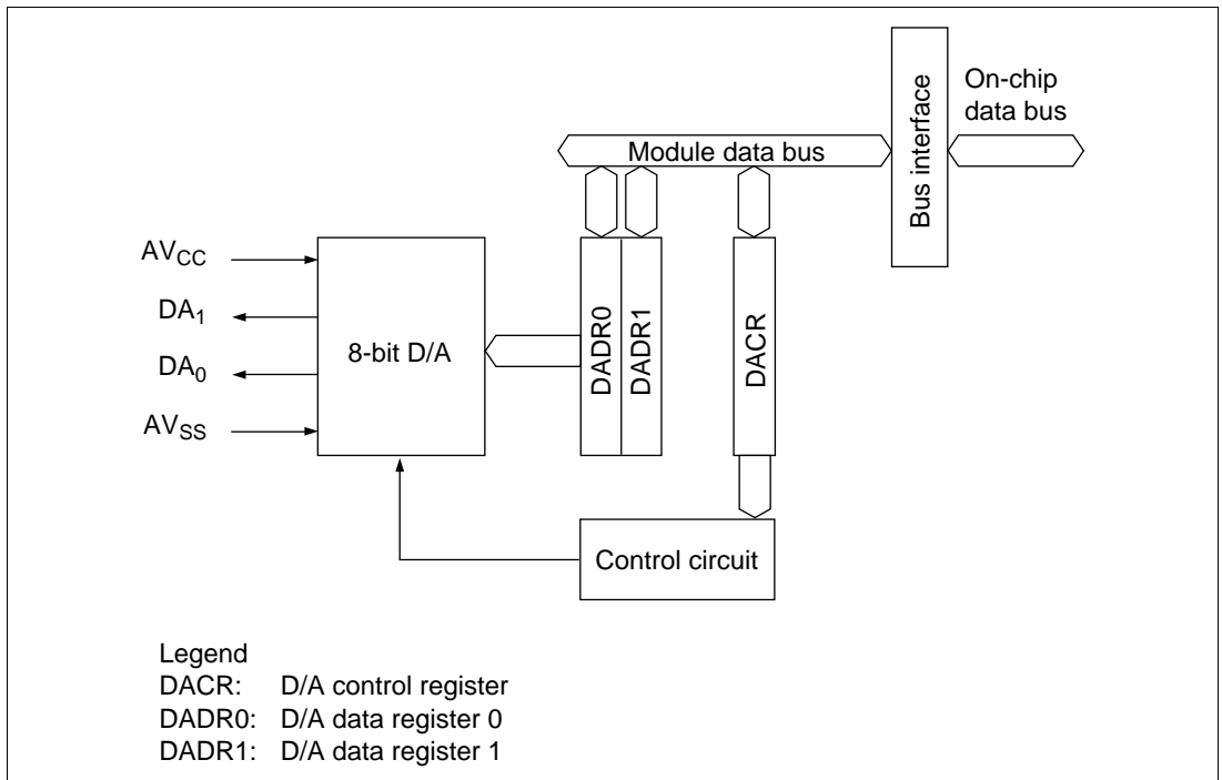
Figure 21.1 Block Diagram of D/A Converter
