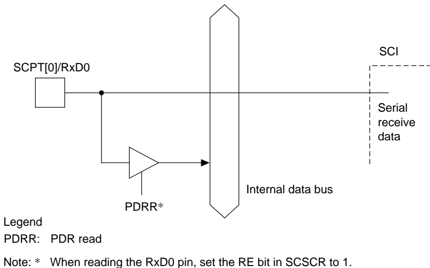
Figure 14.4 SCPT[0]/RxD0 Pin
