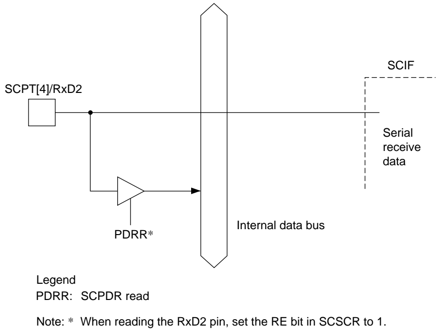
Figure 16.4 SCPT[4]/RxD2 Pin
