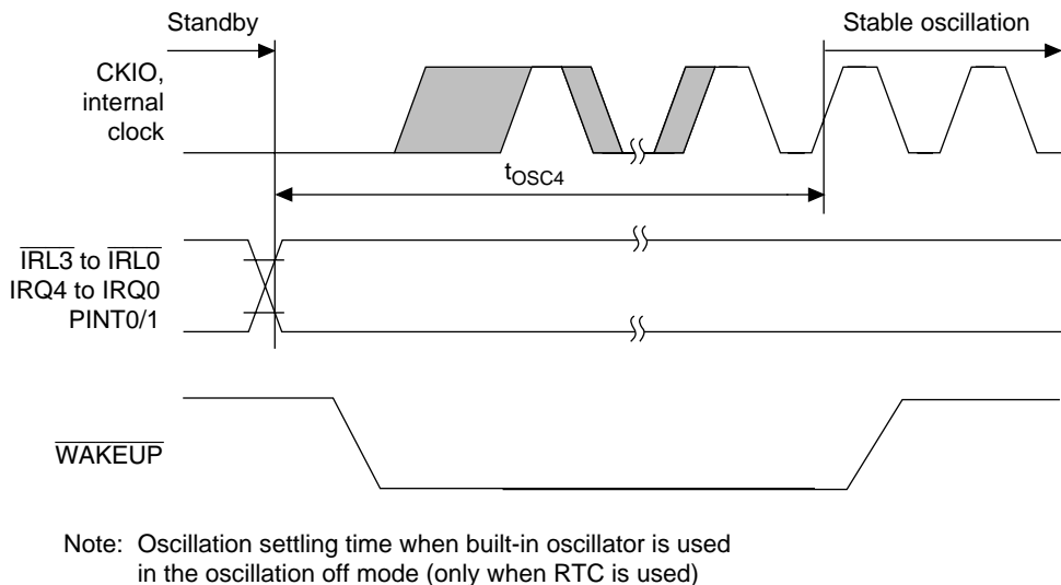
Figure 23.7 Oscillation Settling Time at Standby Return (Return by \overline{IRQ4} to \overline{IRQ0} , \overline{PINT0/1} , \overline{IRL3} to \overline{IRL0} )
