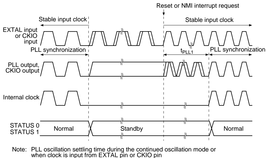
Figure 23.8 PLL Synchronization Settling Time by Reset or NMI
