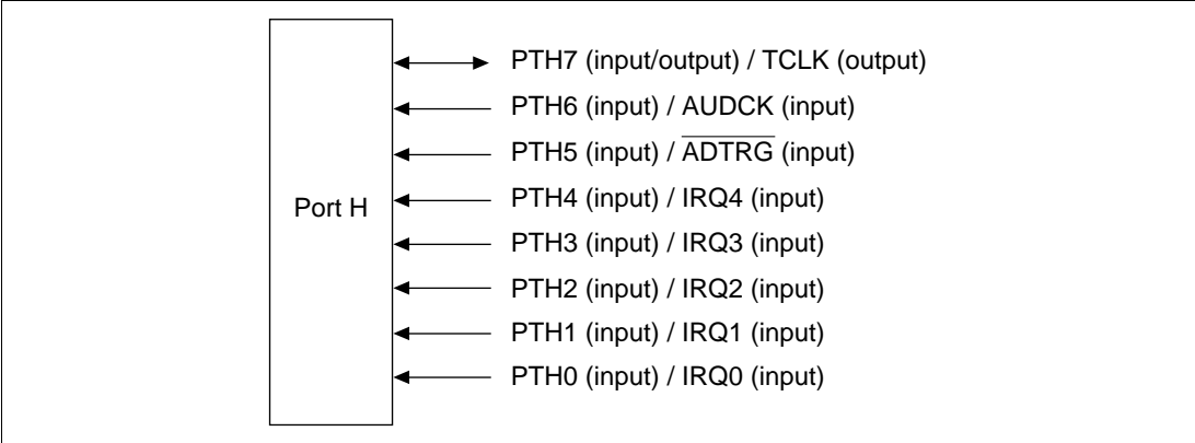
Figure 19.8 Port H
