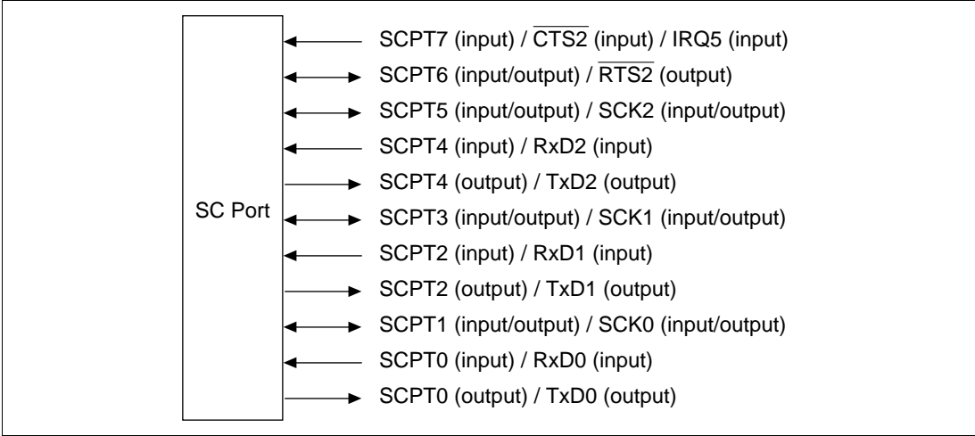
Figure 19.12 SC Port
