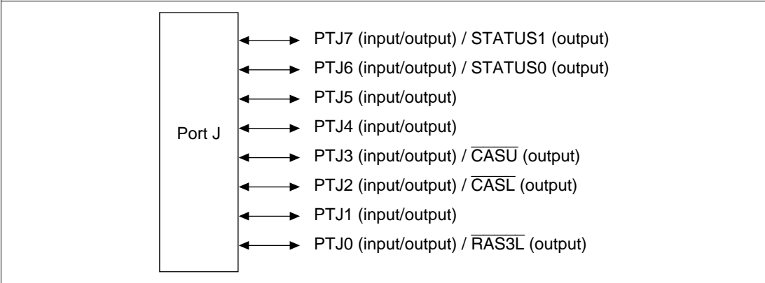
Figure 19.9 Port J
