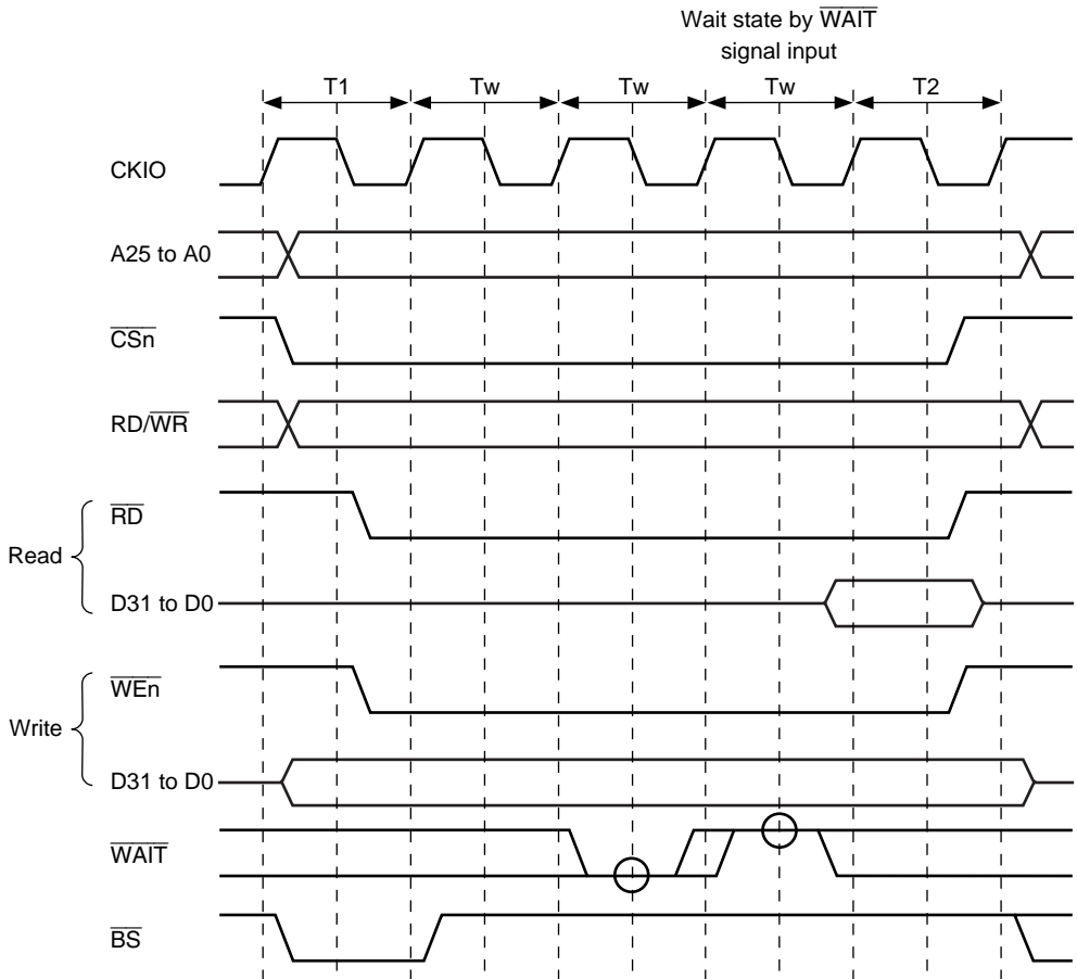
Figure 10.19 Basic Timing for Synchronous DRAM Burst Write
