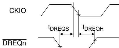
Figure 23.53 \overline{\text{DREQ}} Input Timing
