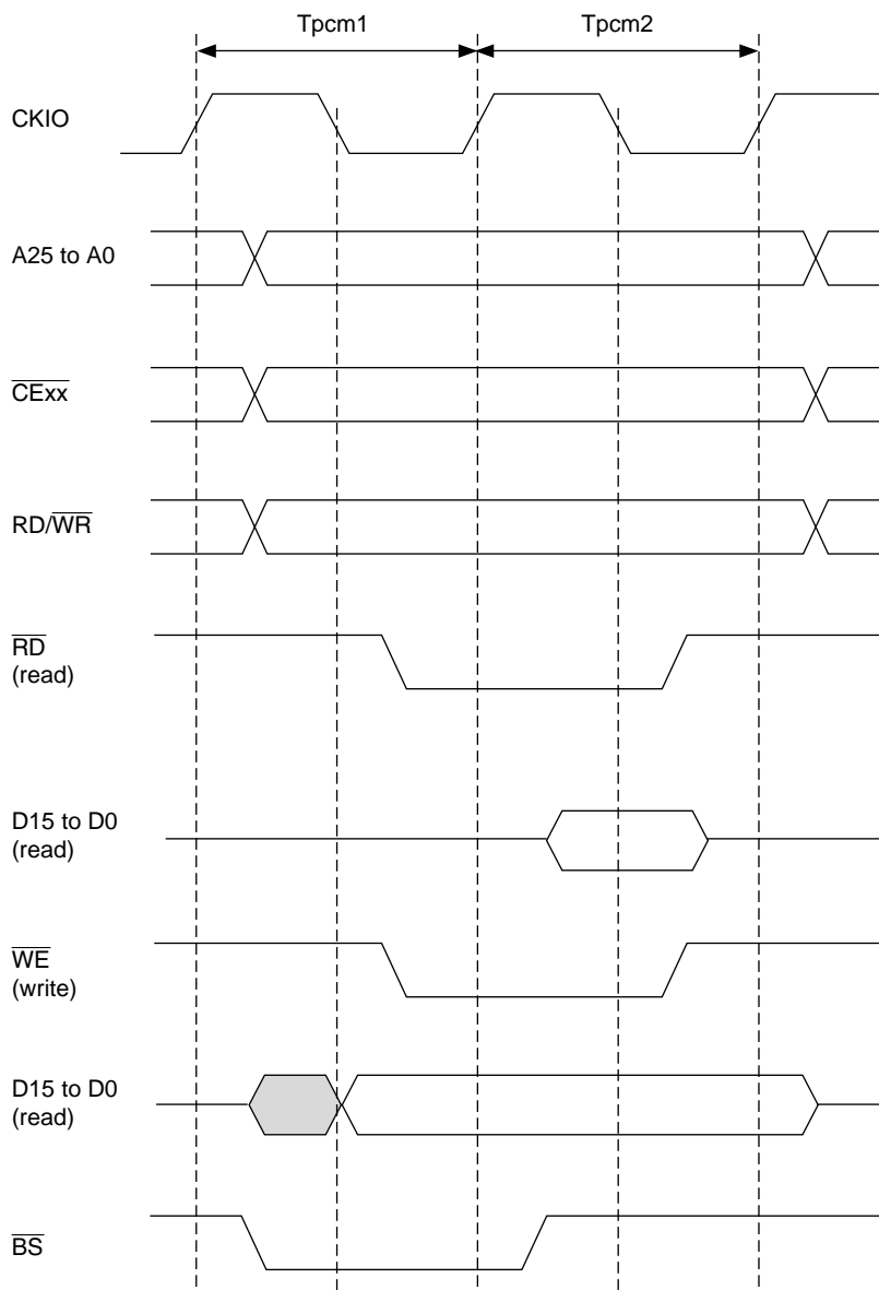
Figure 10.34 Basic Timing for PCMCIA Memory Card Interface
