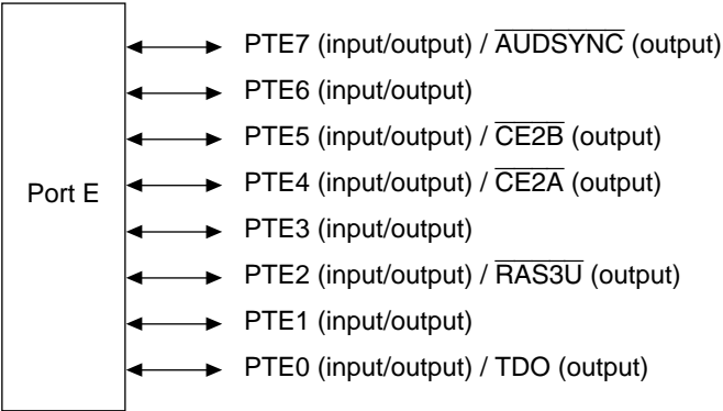
Figure 19.5 Port E
