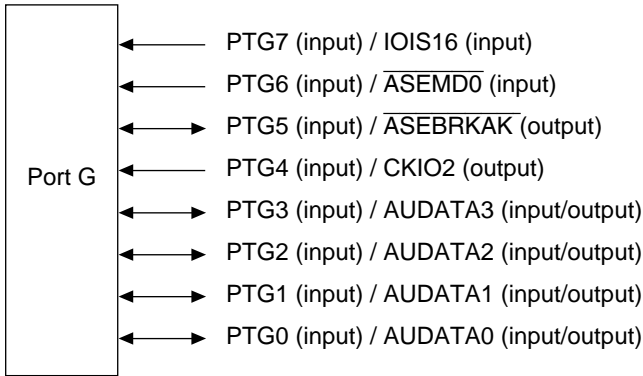
Figure 19.7 Port G
