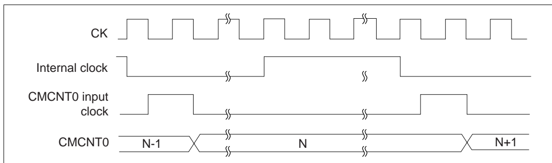
Figure 11.26 Count Timing
