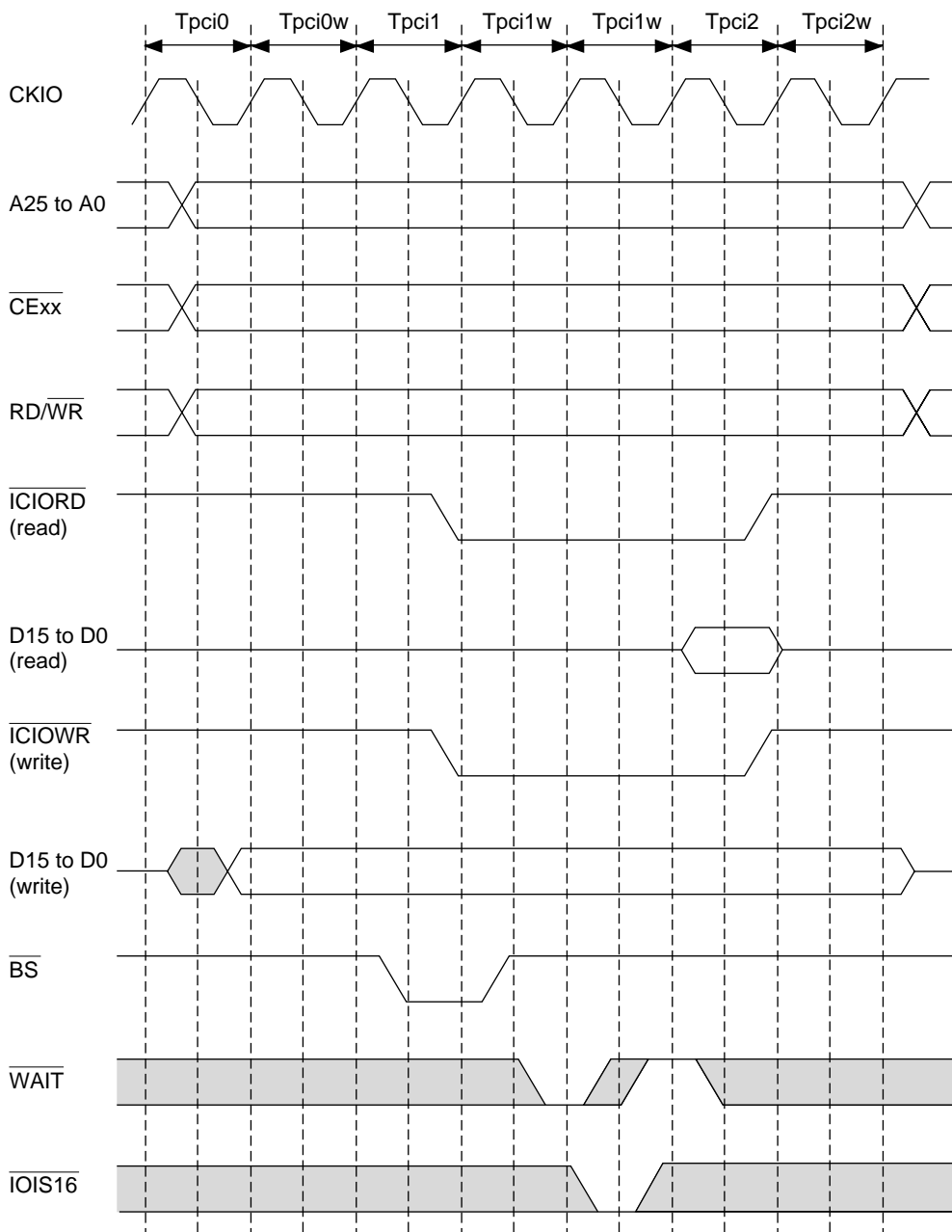
Figure 10.40 Wait Timing for PCMCIA I/O Card Interface
