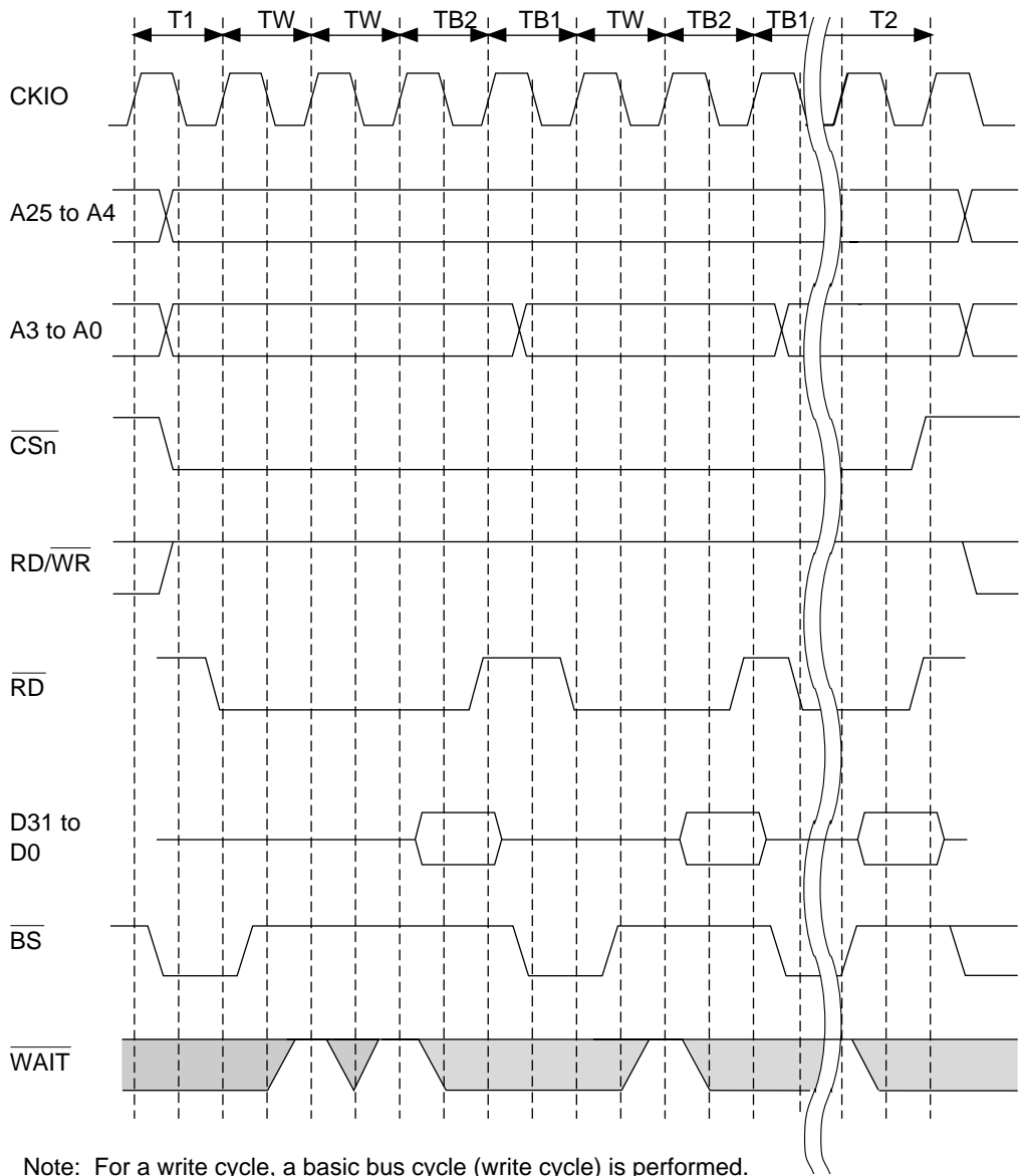
Figure 10.31 Burst ROM Wait Access Timing
