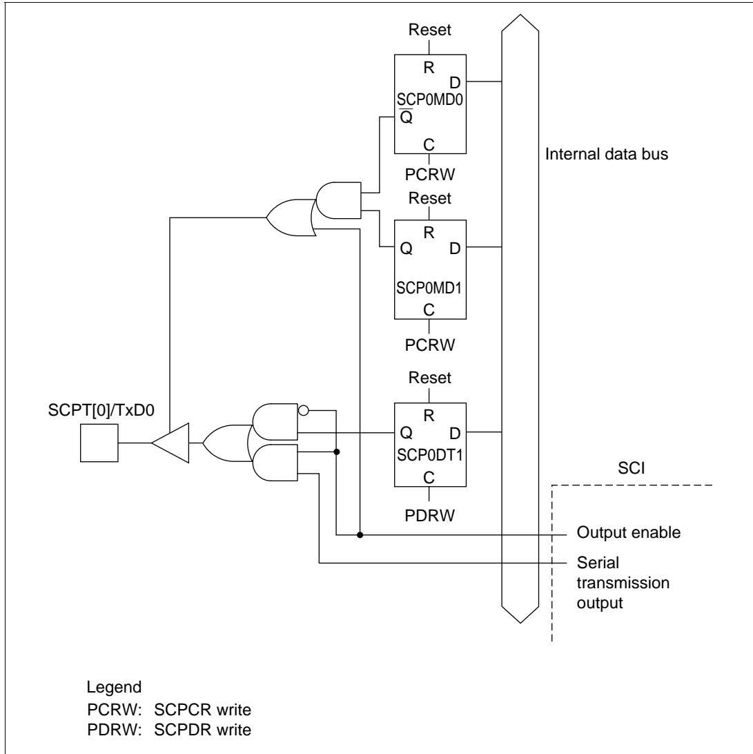
Figure 14.3 SCPT[0]/TxD0 Pin
