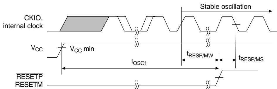
Figure 23.3 CKIO Clock Output Timing
