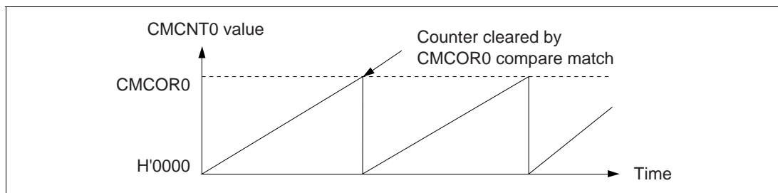
Figure 11.25 Counter Operation
