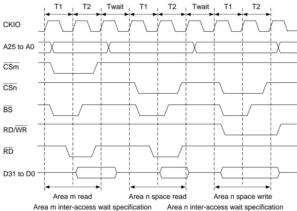
Figure 10.42 Waits between Access Cycles
