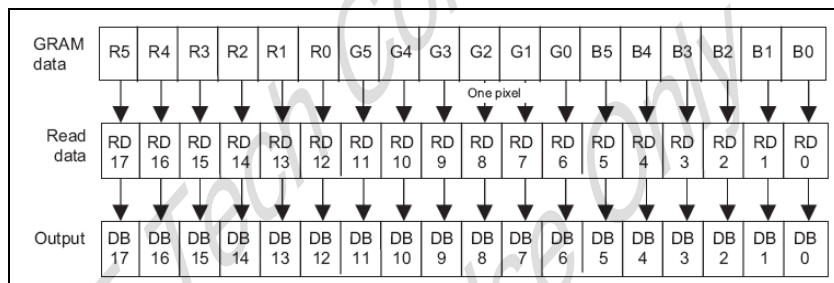
Figure 6.28 18-bit interface
