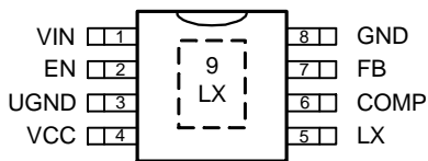
SOP-8P (Top View)
