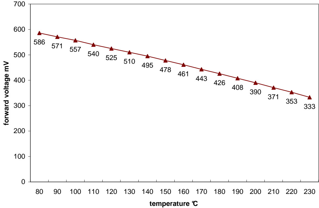
forward voltage 1N4148
