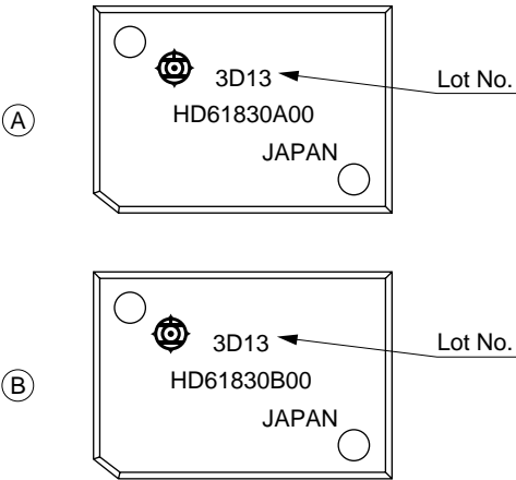
Package Marking
