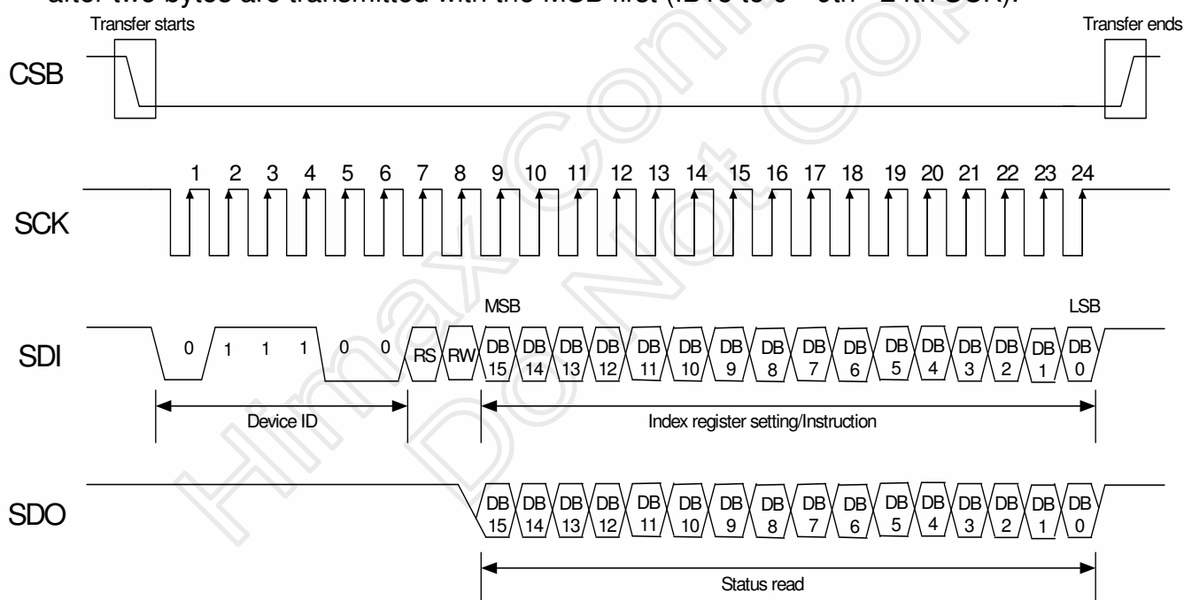
Figure 7.1 SPI Timing
