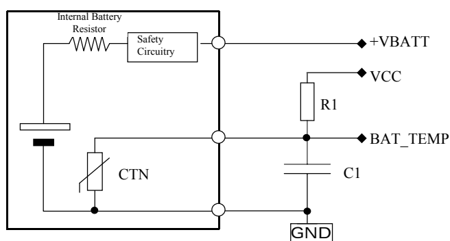
Figure 9 : Connection examples
