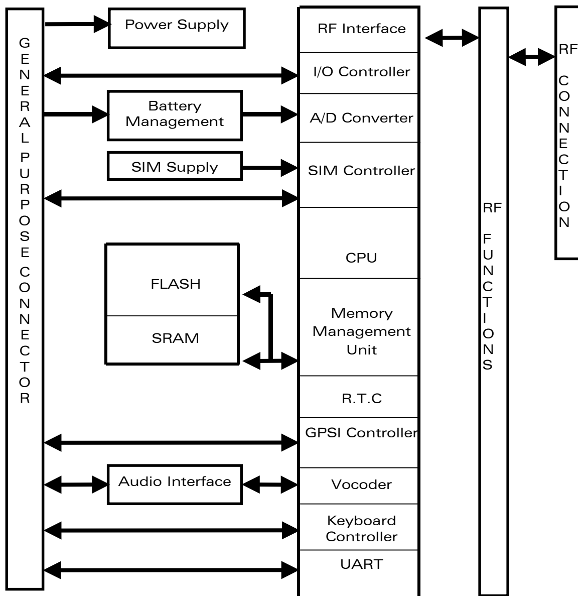
Figure 1 : Functional architecture
