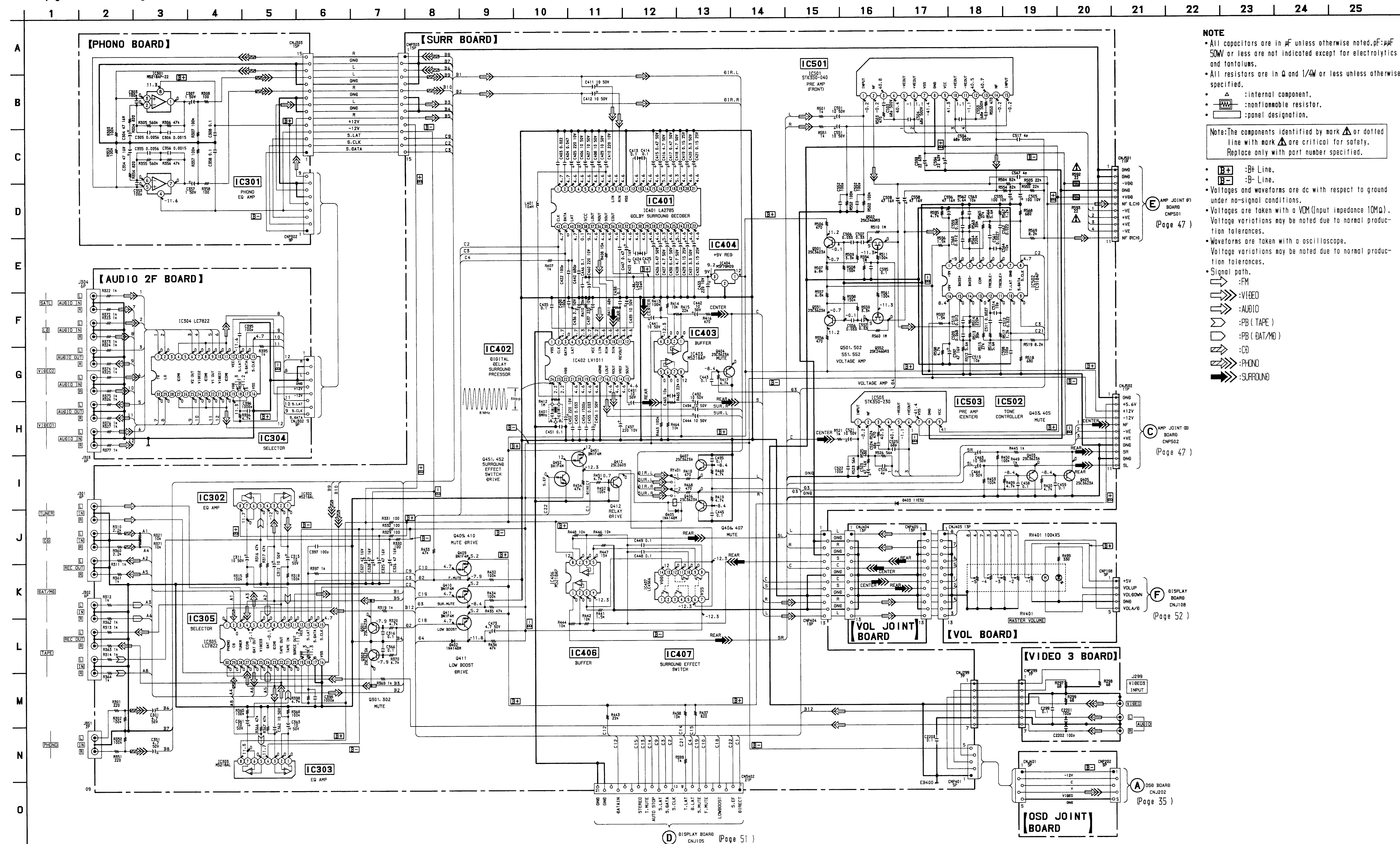
5-3. SCHEMATIC DIAGRAM — SURROUND SECTION — • See page 57 for IC Block Diagrams.
