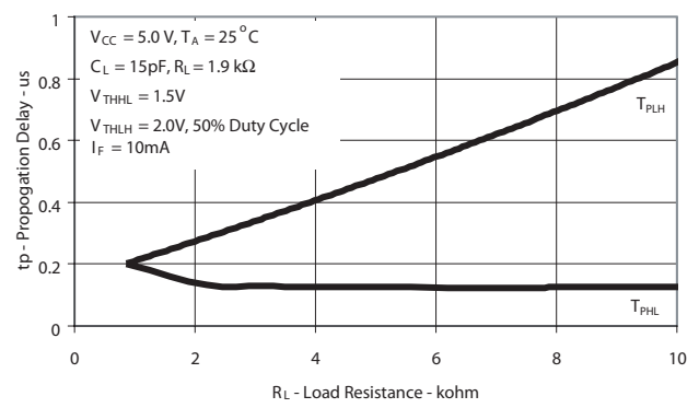
Figure 6. Propagation Delay Time vs Load Resistance
