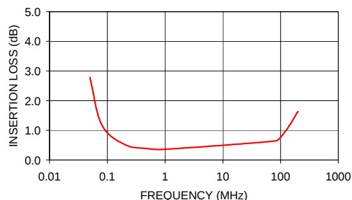
T1-1T-KK81 INSERTION LOSS
