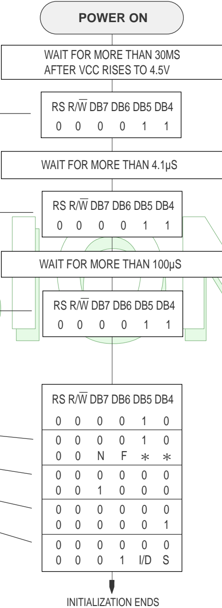
FIGURE2: 4-BIT INTERFACE
