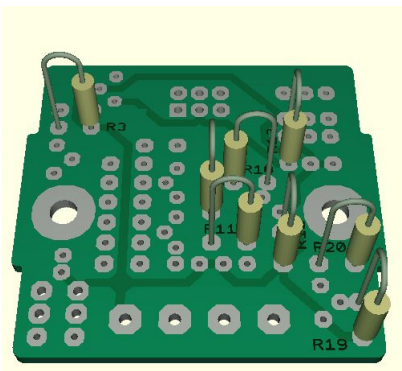
Abbildung 16: R3, R9, R10, R11, R12, R13, R19, R20 (10kΩ)
